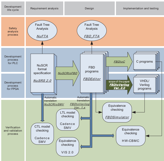
Fig. 1. NuDE (NPP's safety-critical software Development Environment): Software development, verification, and safety analysis for nuclear RPS
