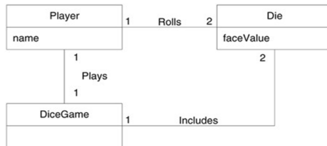
Domain Model
