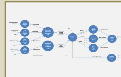
DFD + Process Specifications
