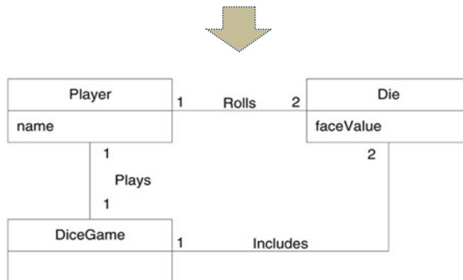
Domain Model
