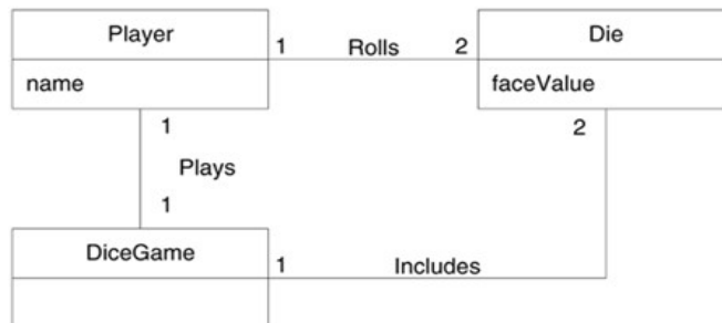
Domain Model
