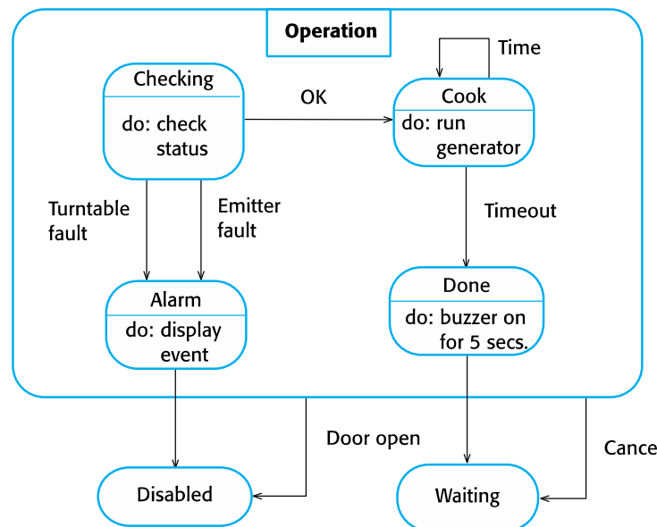
Microwave Oven - Operations State
