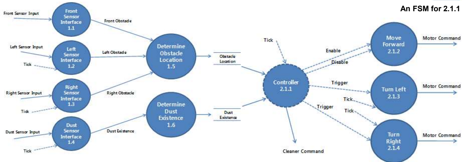
A level 3 DFD for RVC Control
