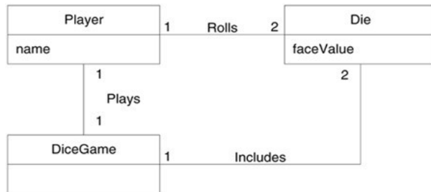
Domain Model
