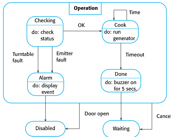
Microwave Oven - Operations State
