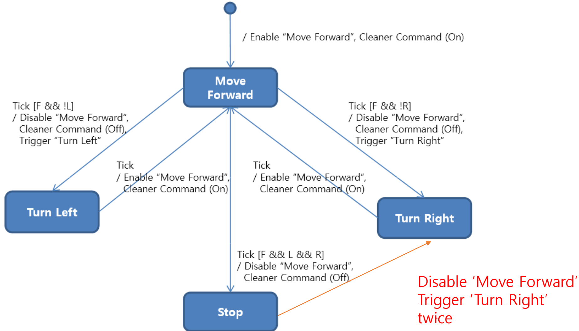
State Transition Diagram for Controller 2.1.1
