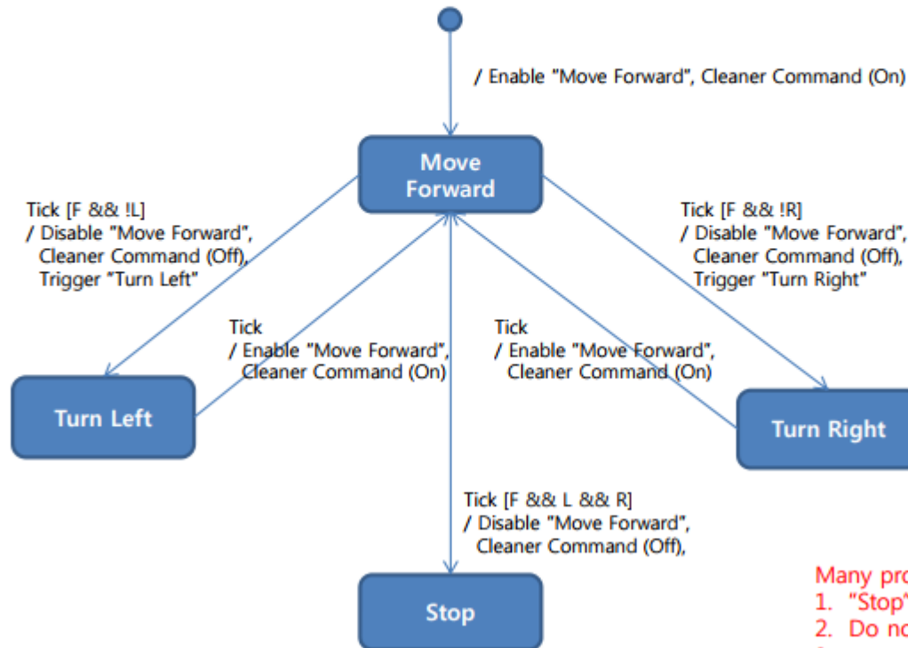
State Transition Diagram for Controller 2.1.1
