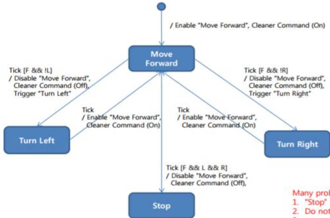
State Transition Diagram for Controller 2.1.1
