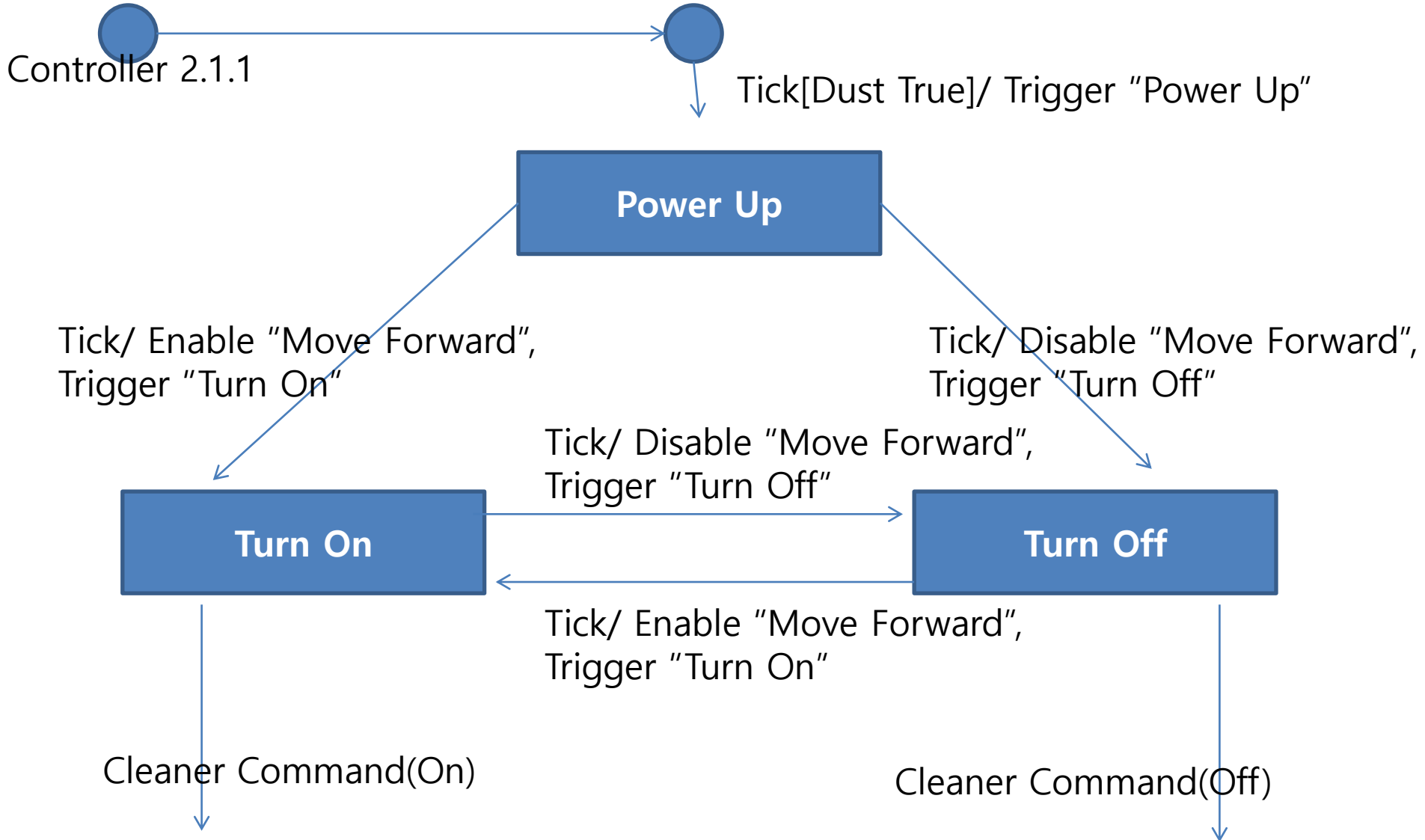
Diagram for Dust Controller 2.1.5
