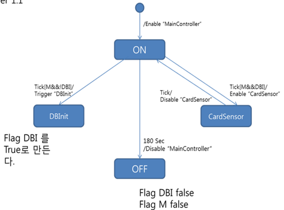
State Transition Diagram for Controller 1.1
