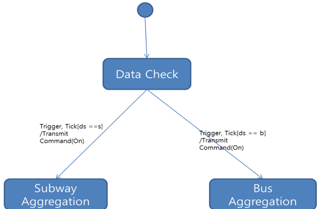
State Transition Diagram for Aggregation Controller 3.1
