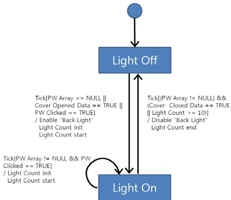
3.2.4.4.4 State Transition Diagram for Light Controller(2.2.2)
